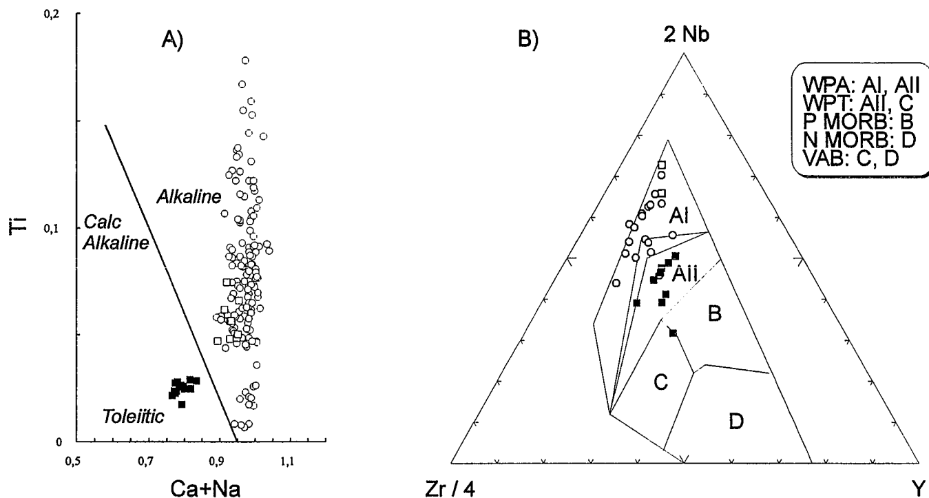
Figure 2.- A) Ca+Na vs Ti diagram (Letterrier et al. , 1982) for pyroxenes from basic magmatic rocks in the Almadén district. Open circles: Basalts; black squares: dolerites; field A: pyroxenes from alkaline rocks; field CA: pyroxenes from calc-alkaline rocks; field T: pyroxenes from tholeiitic rocks. B) 2Nb:Zr/4:Y Diagram (Meschede, 1986) for the whole rock composition of basic magmatic rocks of the Almadén district. WPA: Within-plate alkaline basalts; WPT: Within-plate tholeiites; P MORB, N MORB: Mid-ocean ridge basalts; VAB: Volcanic arc basalts. Symbols, as in figure 2A.
