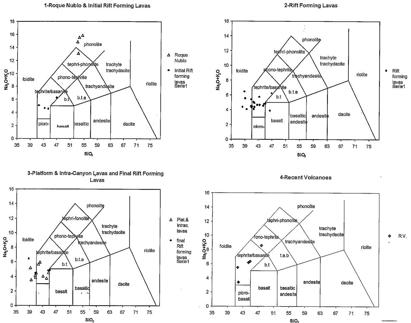
Fig. 2.- TAS classification of studied rocks arranged from older to recent ones (2.1 to 2.4, see text for explanation)
