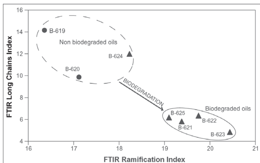
Fig. 4.- The non biodegraded sample B624 shows a more elevated value of Long Chains than other oils from the same group (B621 to B625) in Figure 3. Note that samples B619 and B620 are also non biodegraded.
