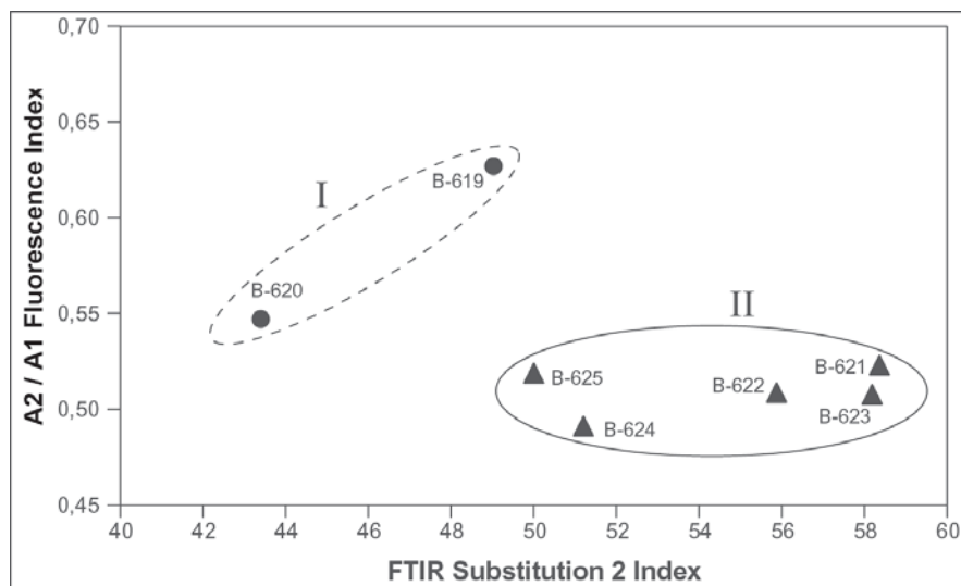
Fig. 2.- Fluorescence A2/A1 vs. FTIR Substitution 2 indexes clearly evidence two groups of oils.
