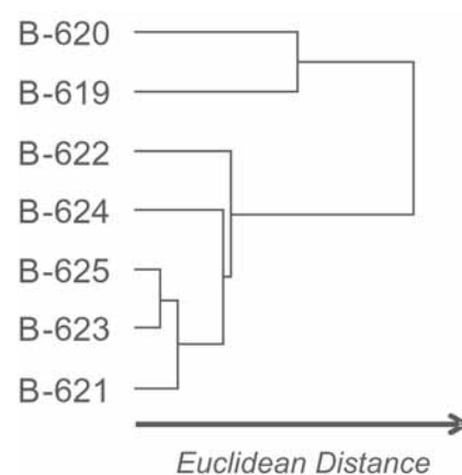
Fig. 3.- Cluster analysis using biomarkers ratios evidences two groups of oils.
