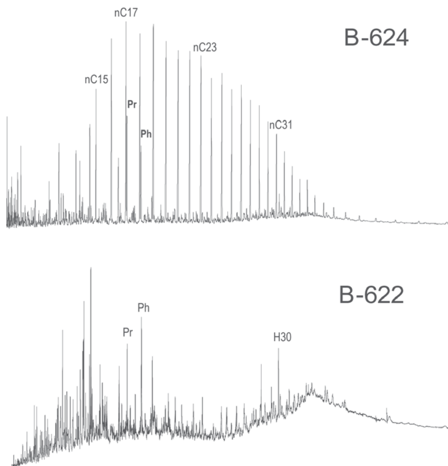
Fig. 1.- Whole oil CG/FID chromatograms of two oil samples from the same field in a Brazilian Basin, showing distinct biodegradation degrees. Sample B-622 is the most biodegraded.
